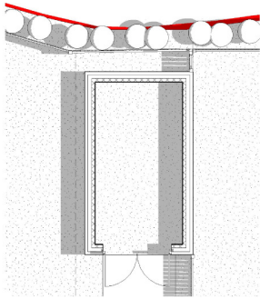
1 01 Ground Floor Plan - Callout Garage 1:50
