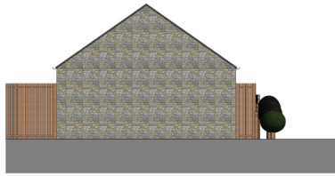
5. Garage Elevation 3 1:50
