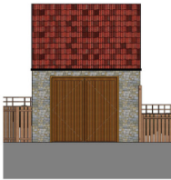
4. Garage Elevation 2 1:50
